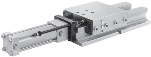
For dimensions not shown, see "HWL" basic assembly on page 15.
