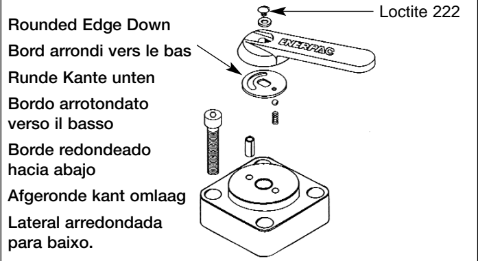
Handle Assembly
